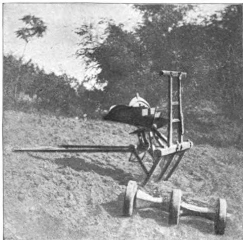
A CHINESE SEEDING-DRILL.
